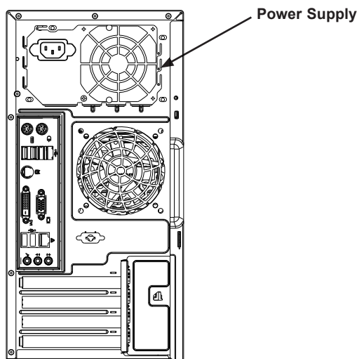
Figure 4-13: Removing the Power Supply
