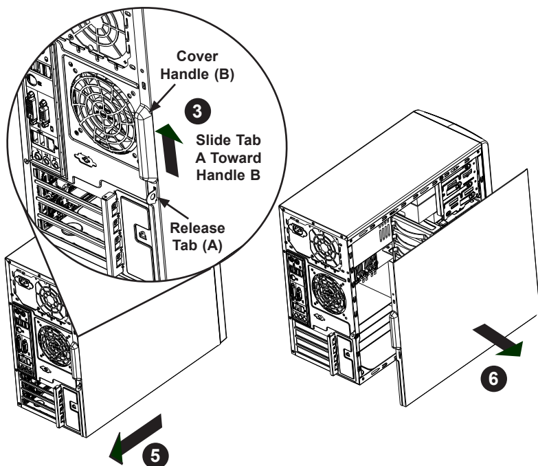
Figure 4-1: Removing the Chassis Cover
