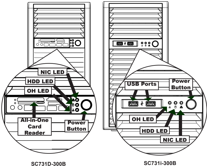
Figure 3-1: Front Chassis Panels
